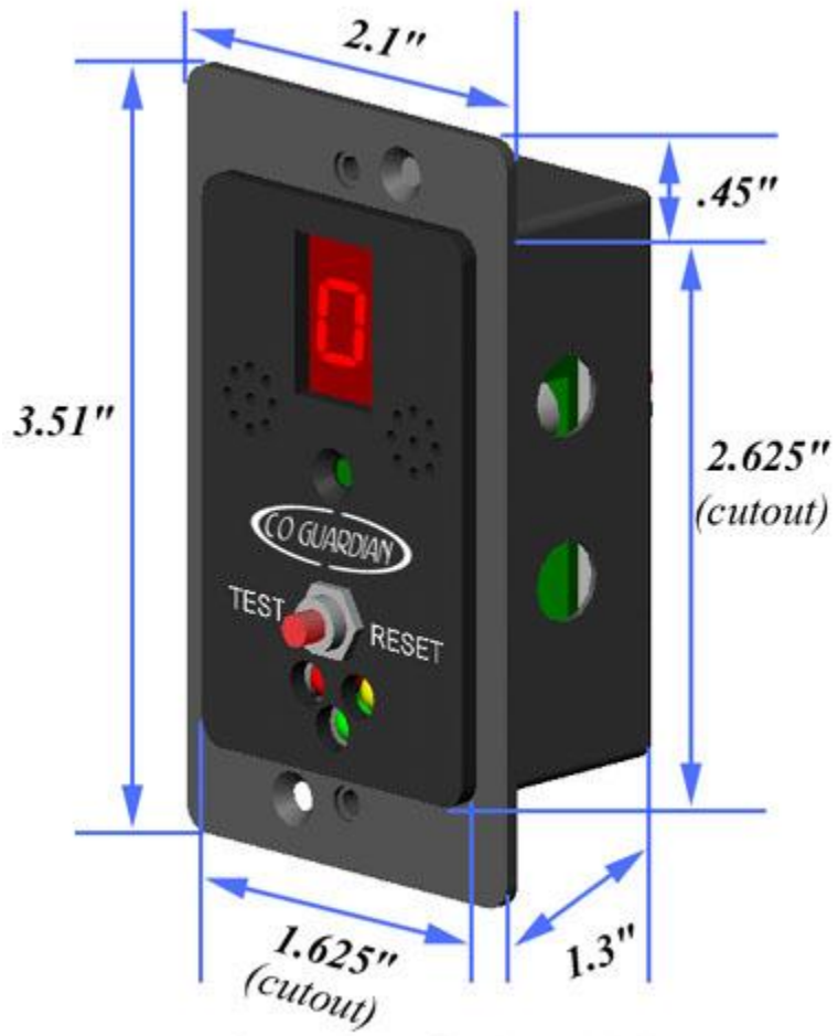
Dimensions for Aero-252
